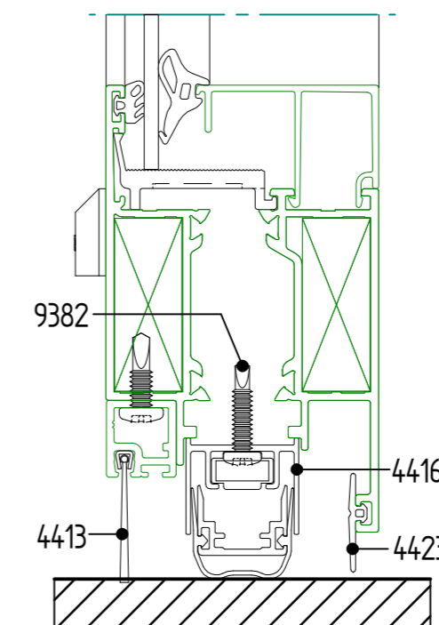
Drop seal option
